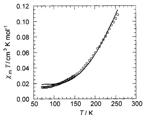
Fig. 4 Plot of \chi T vs. T for [\text{Cu}(\text{fsaaep})(\text{H}_2\text{O})]_2 2 .
