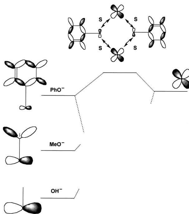
Fig. 6 Schematic representation of the antagonistic effects of the energy difference between the MOs of the fragments and their overlap (see text).
