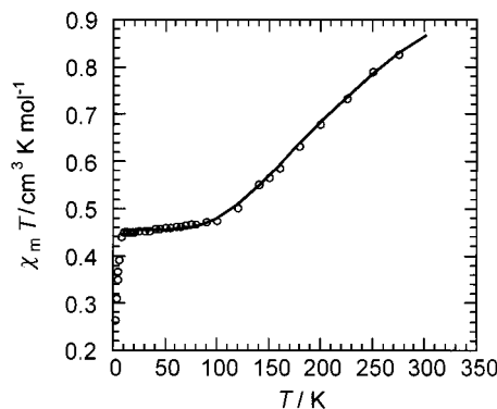
Fig. 5 Plot of \chi T vs. T for the trinuclear complex [\text{Cu}_3(\text{fsaaep})_2][\text{ClO}_4]_2 3 .
