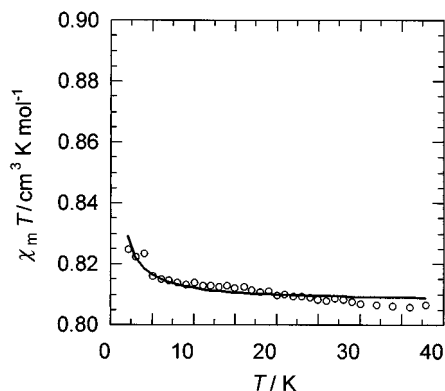
Fig. 3 Plot of \chi T vs. T for [\text{Cu}(\text{Hfsaaep})\text{Cl}]_2 1 .
